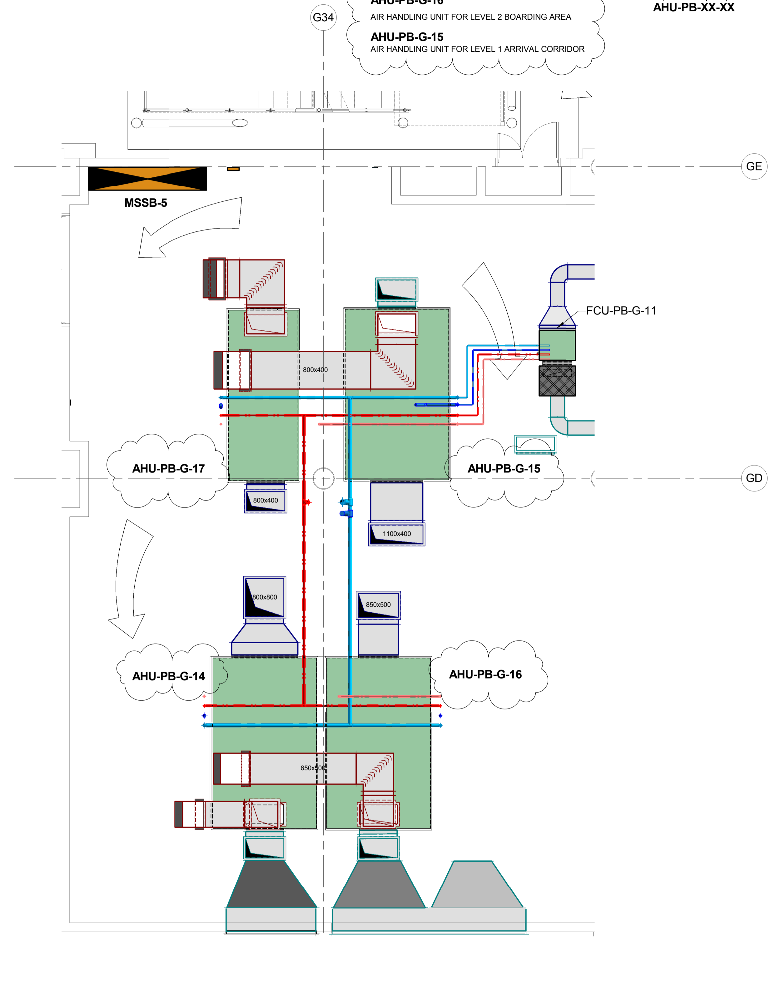
GATE 18 MECHANICAL PLANT - LOW LEVEL
