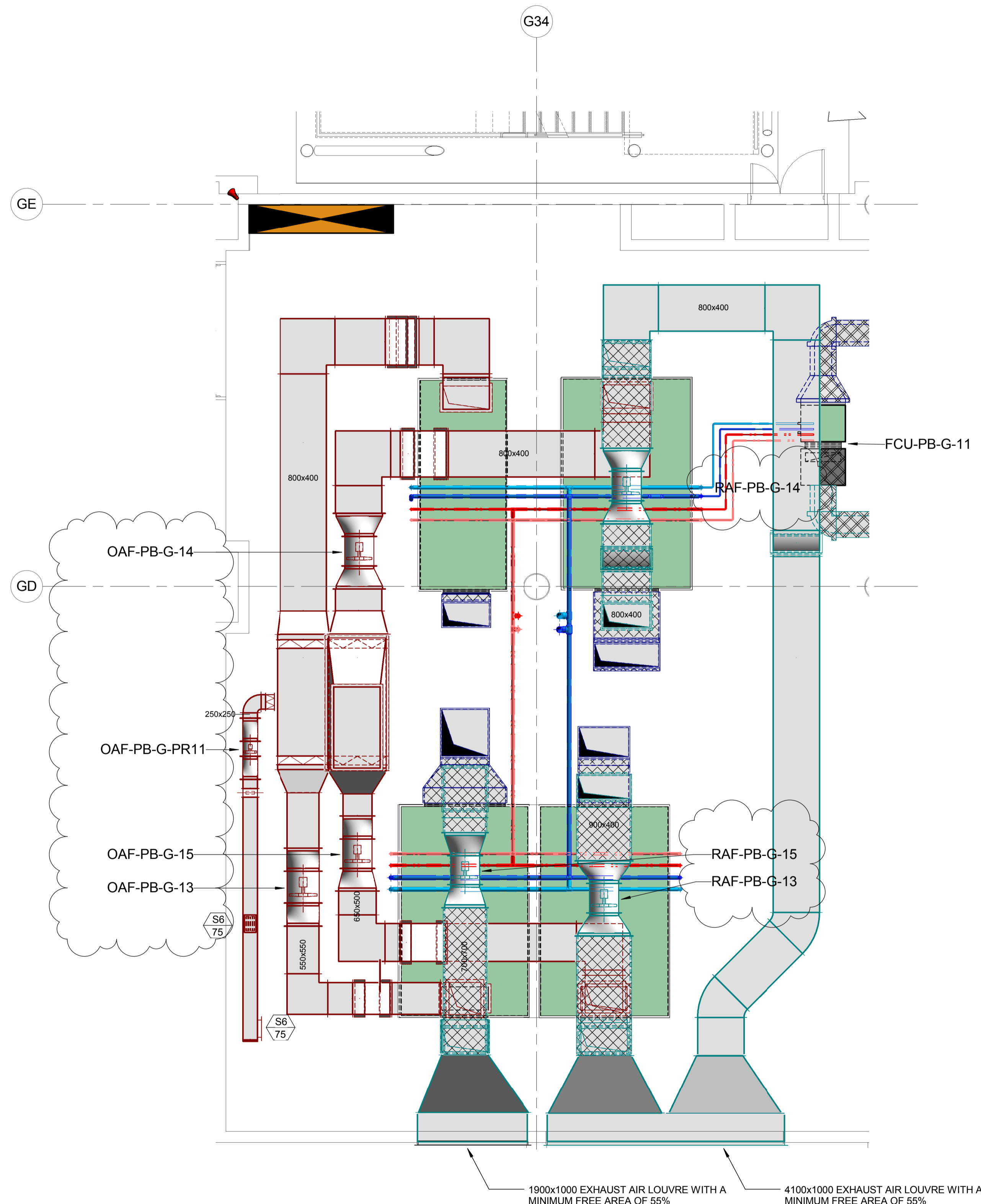
GATE 18 MECHANICAL PLANT
