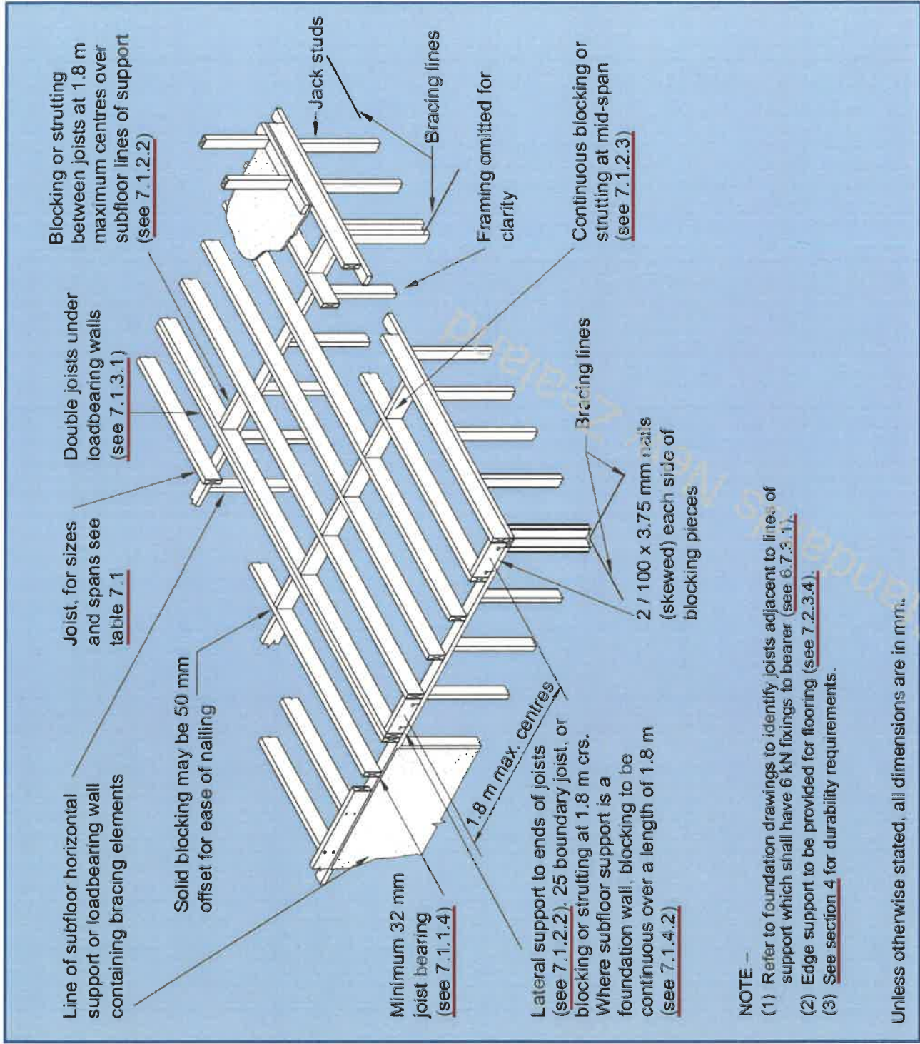
Figure 7.2 – Floor joists layout criteria (see 7.1.2.2)
