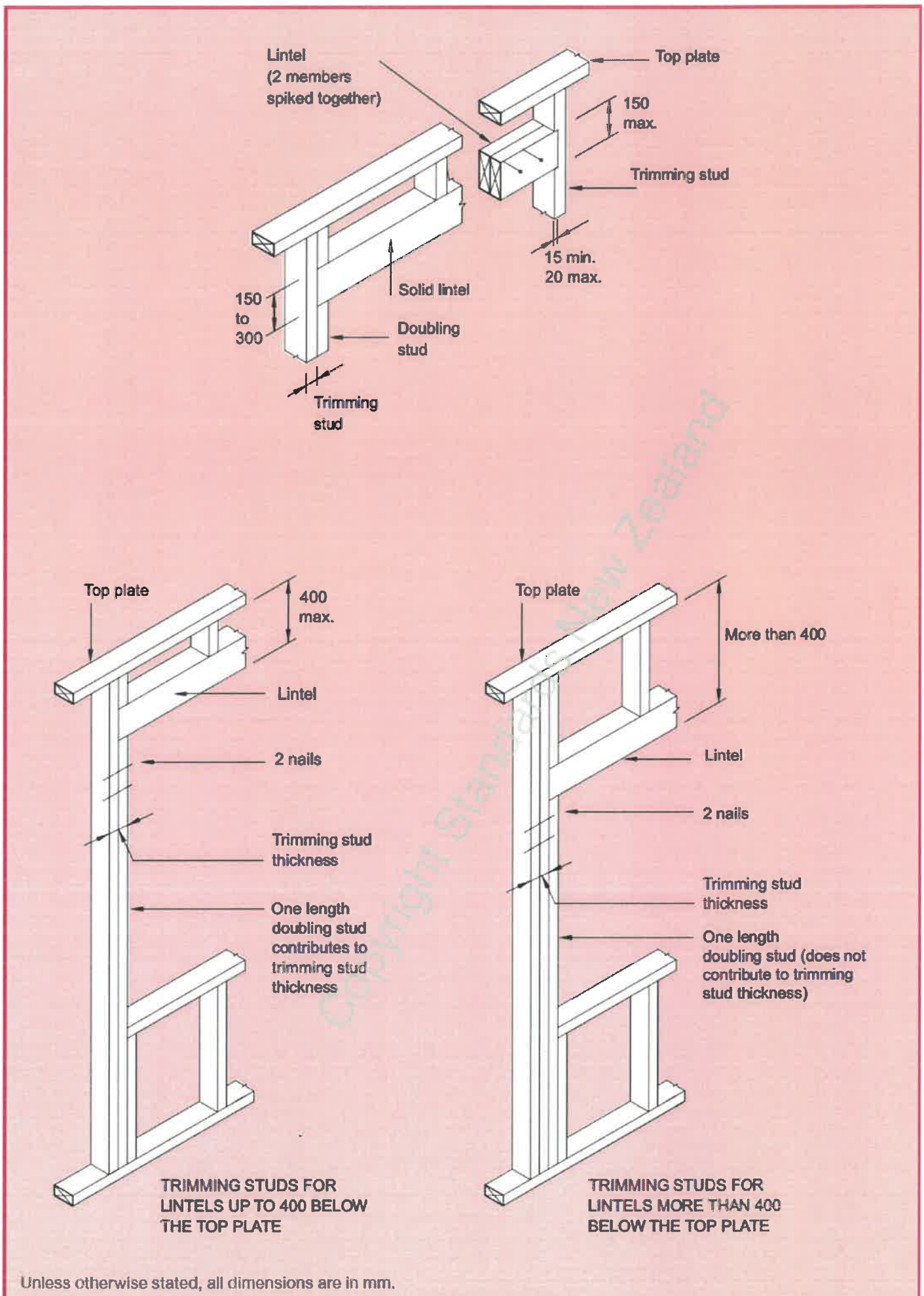
Figure 8.5 – Trimming studs and lintels (see 8.5.2.1)
